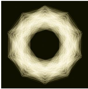
Azimuth of the Sun
